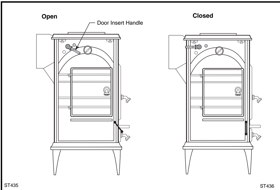
Fig. 23 Damper operating positions.
