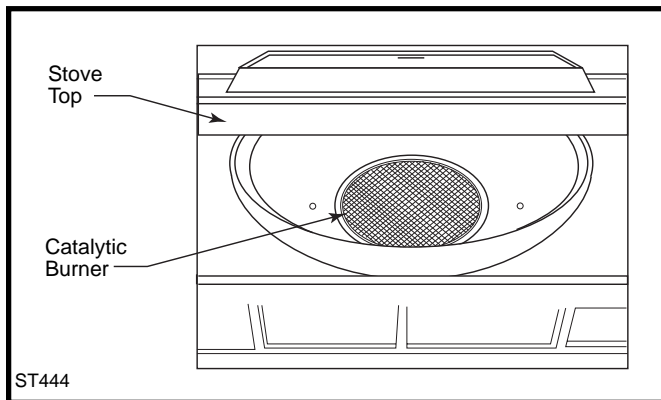
Fig. 31 Remove refractory package with care.
