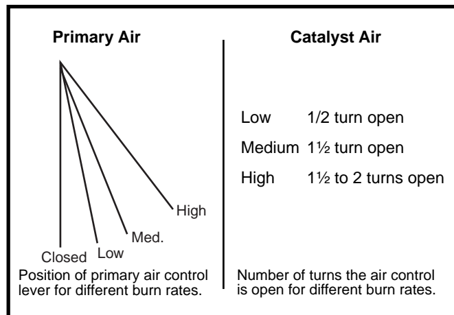
Fig. 24 Primary and Catalyst air settings.
