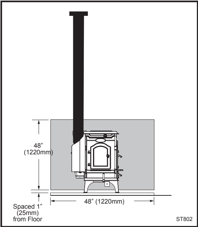
Fig. 22 Sidewall protection.
